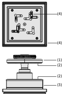
System Design Mechanical clamps VCMC-R-QUICK
